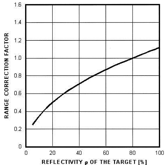
Fig. 5. Correction factor for maximum laser range, depending on target reflectivity (lasers of firm Riegler, 900 nm wavelength, diffuse targets, maximum range in the specifications given for 80% reflectivity).
