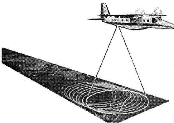
Fig. 10. Progressing Palmer scan.
