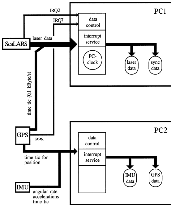
Fig. 11. Synchronisation of laser scanner (ScaLARS), GPS and IMU.
